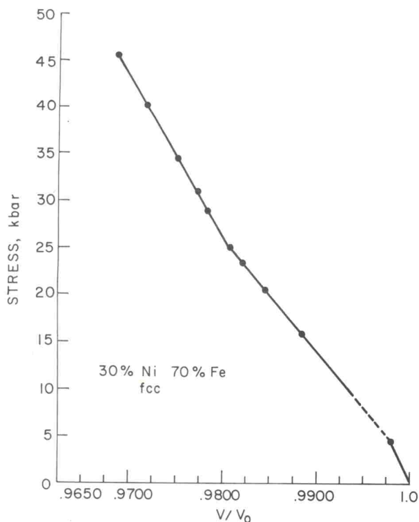
Fig. 12 Stress-volume relation observed for fcc 30%Ni-70%Fe
